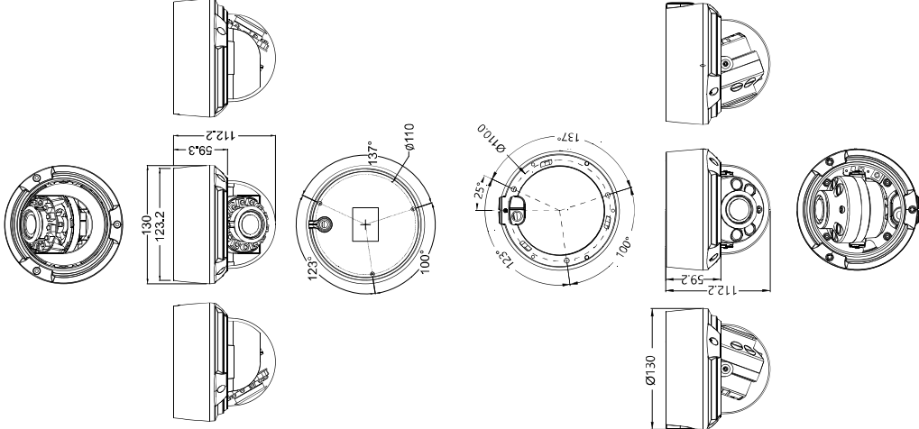
Figure 2-2 Dimensions ( Unit:mm )
