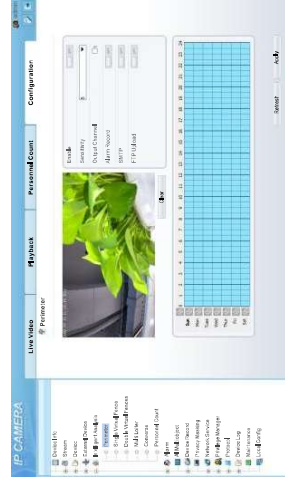
Figure 4-7 Intelligent Analysis
