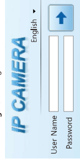
Figure 4-1 Login
